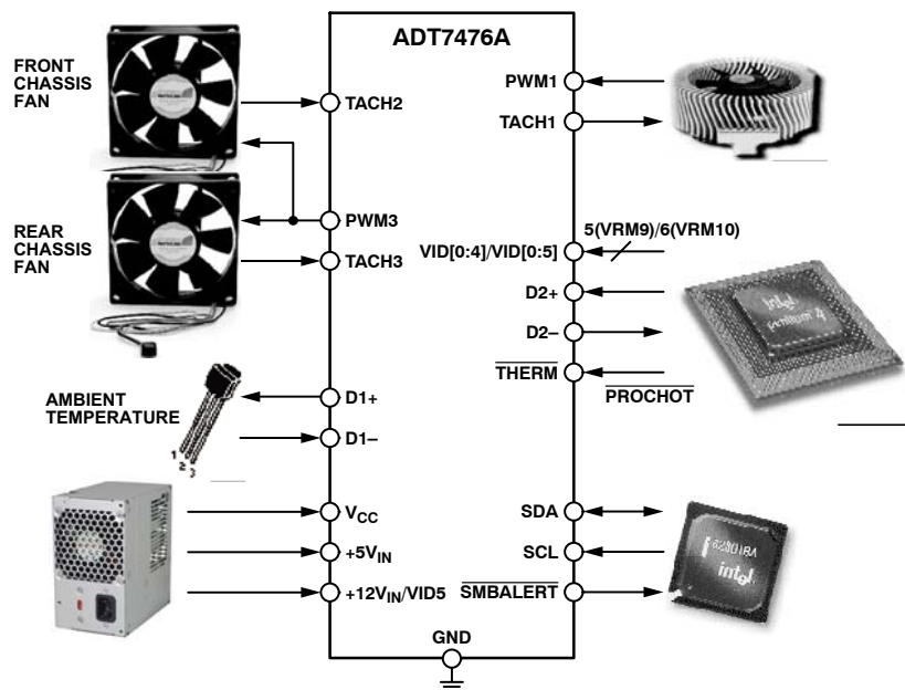
Figure 13. ADT7476A Configuration
